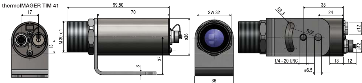
thermoIMAGER TIM 41
